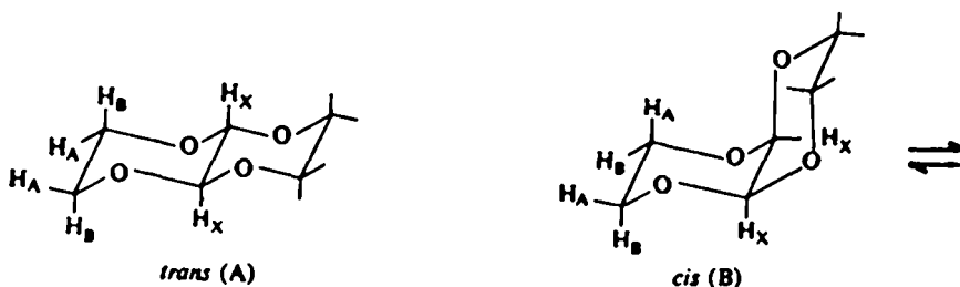
FIG. 2. Two possible structures of 1,4,5,8-naphthodioxans.
